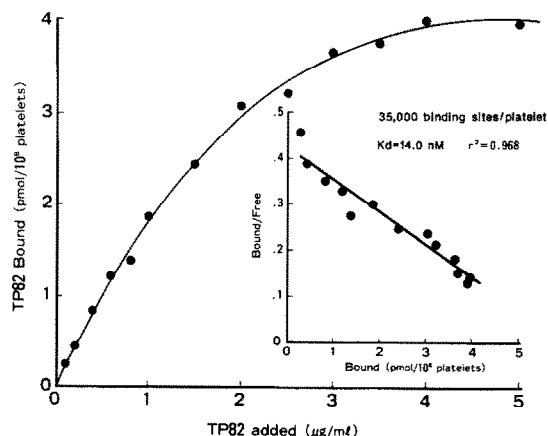
Fig. 1. 125 I-TP82 IgG binding on human platelets. 5 × 10 7 platelets were incubated with 125 I-TP82 antibody for 30 min at 22°C. The inset represents a Scatchard plot of the binding data.
